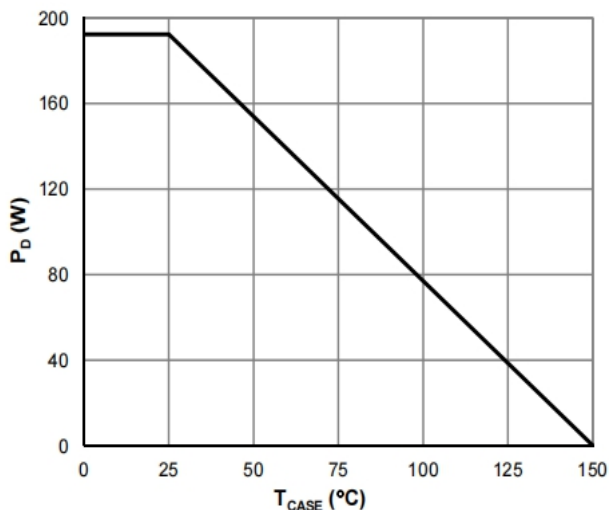
Figure 10: Power De-rating
